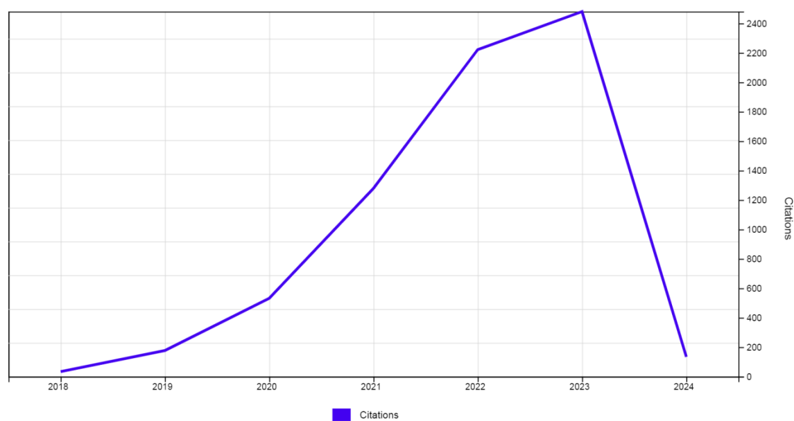
Figure 7 Citations
