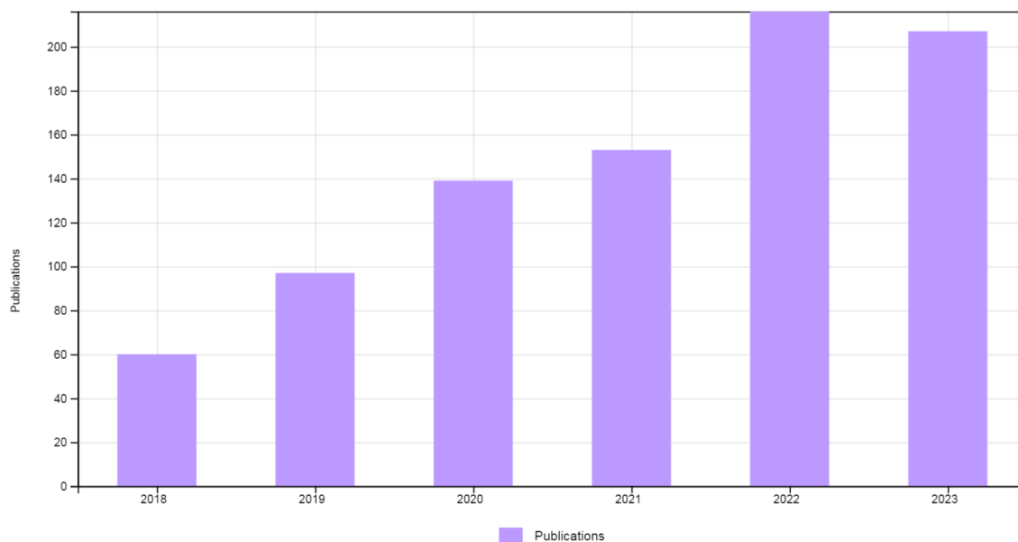
Figure 6 Publications
