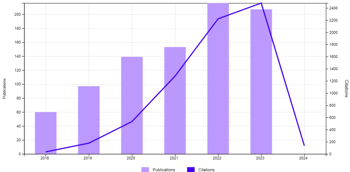
Figure 5 Publications
